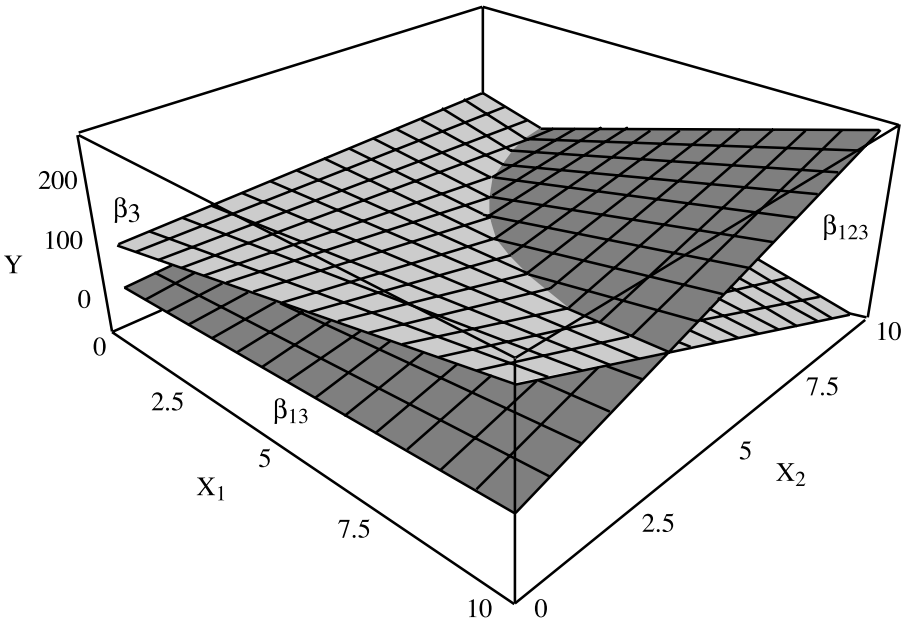
FIGURE 1. y = \beta_0 + \beta_1x_1 + \beta_2x_2 + \beta_3x_3 + \beta_{12}x_1x_2 + \beta_{23}x_2x_3 + \beta_{13}x_1x_3 + \beta_{123}x_1x_2x_3 at two different levels of X_3 , showing the impact of \beta_3 , \beta_{13} , and \beta_{123} .
